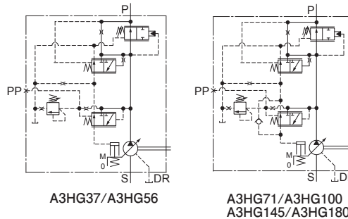
Graphic Symbols
