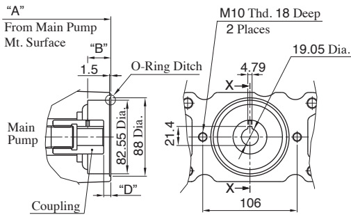
Section X-X
