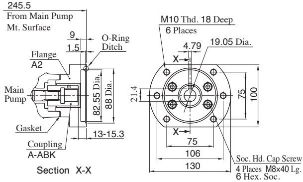
Section X-X
