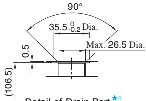
Detail of Drain Port ★4
